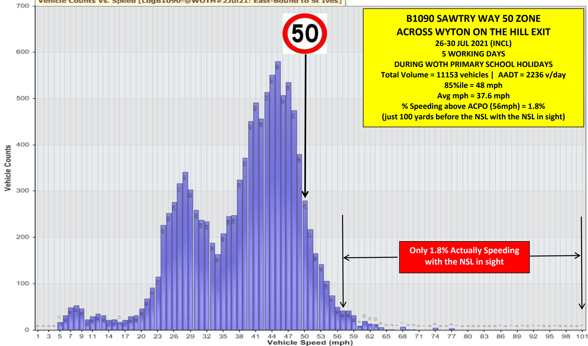
Vehicle Counts Vs. Speed [LogB1090-@WOTH#2Jul21: East-Bound to St Ives]
