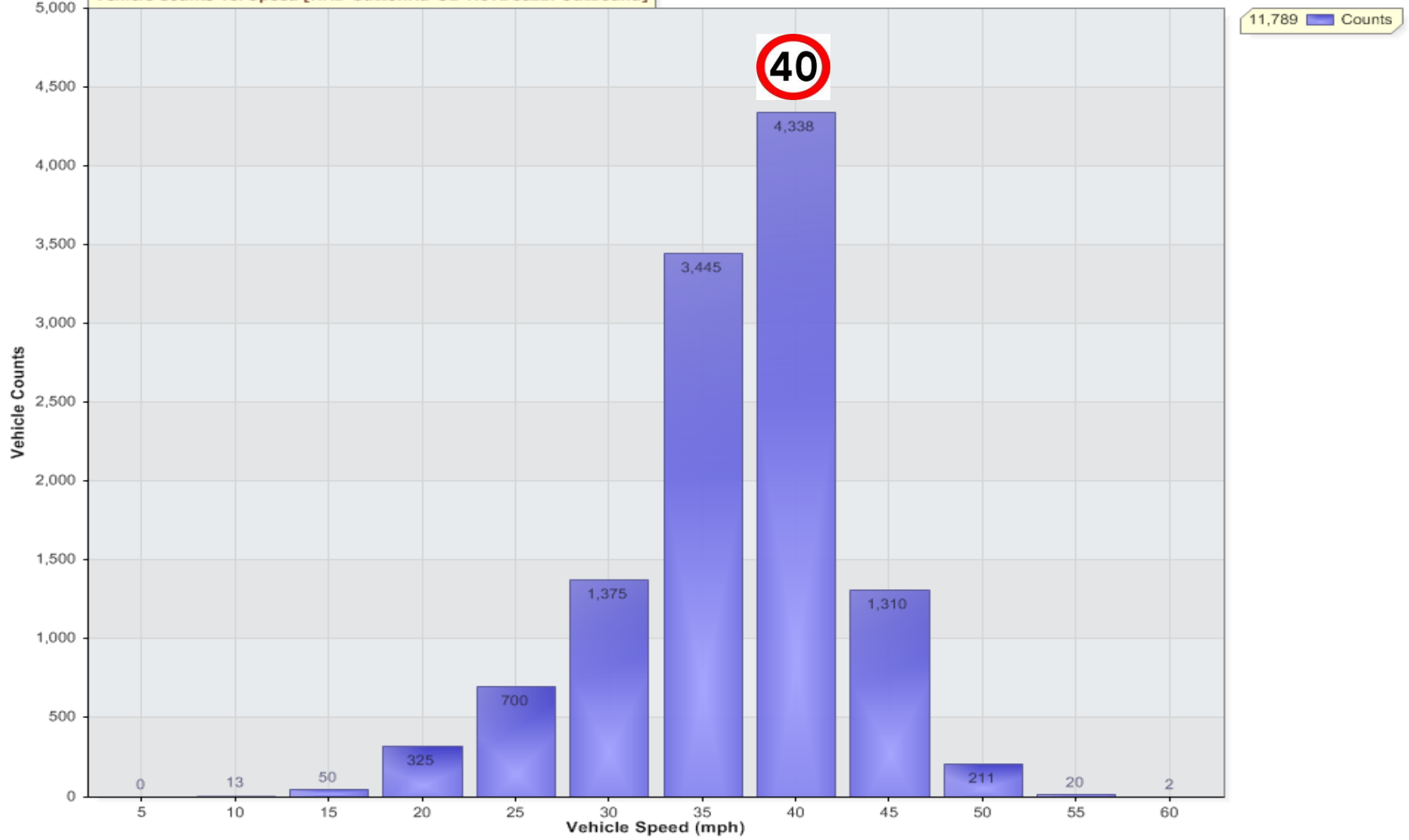
Vehicle Counts Vs. Speed [HAD-SuttonRd-OB-NovDec21: Outbound]
