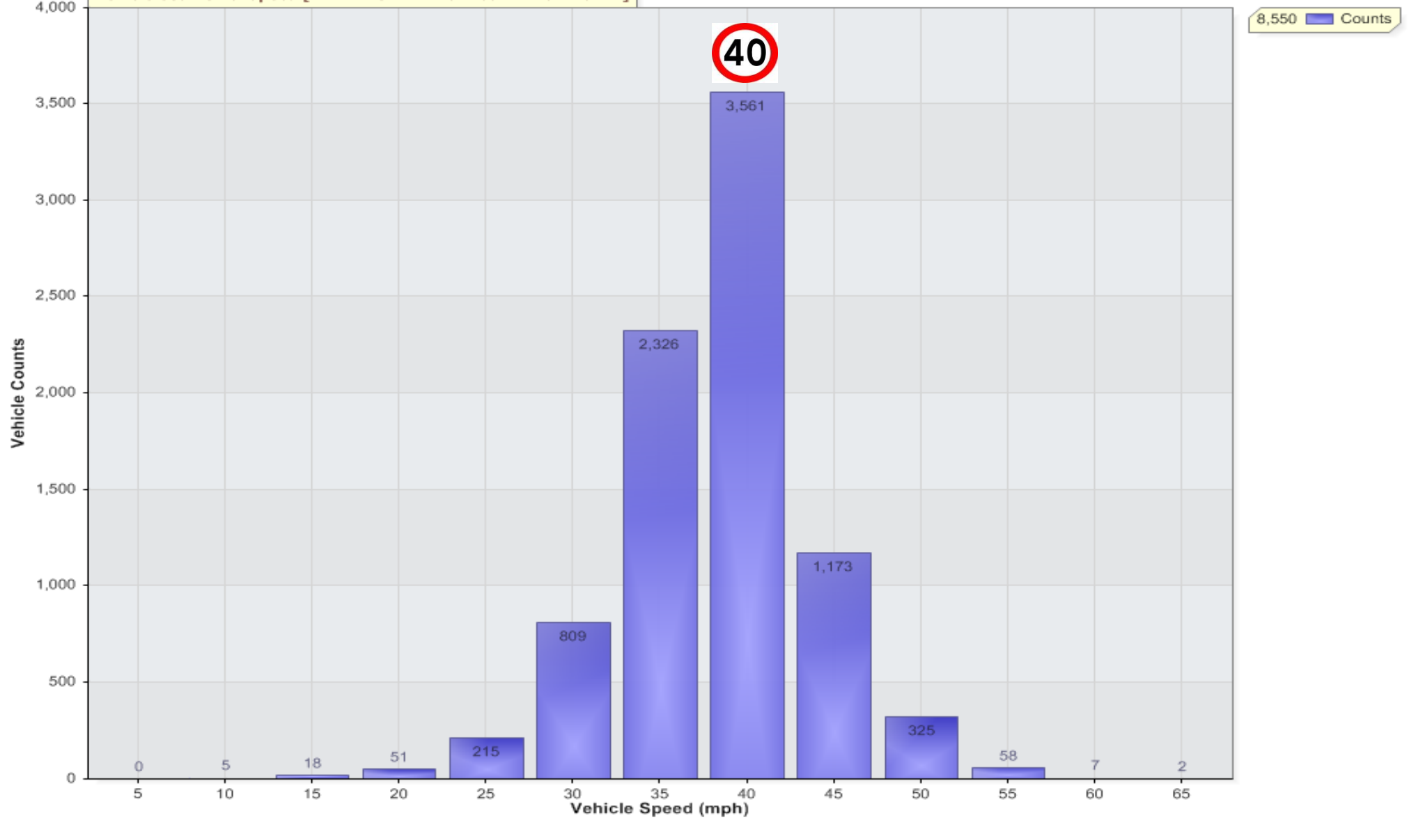
Vehicle Counts Vs. Speed [HAD-HRow-IB-NovDec21: From Earith]
