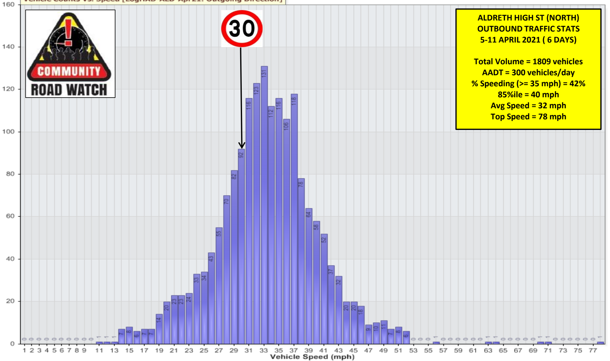
Vehicle Counts Vs. Speed [LogHAD-ALD-Apr21: Outgoing Direction]
