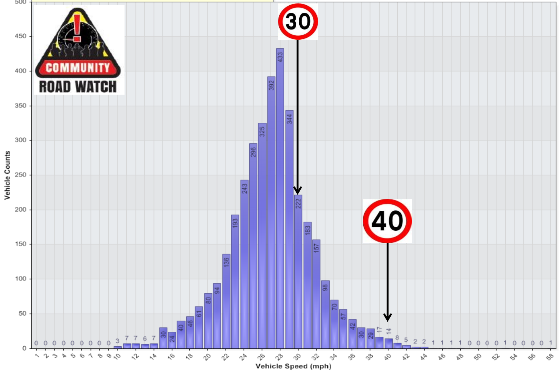
Vehicle Counts Vs. Speed [LogELS-BoxRdAtGnD-Apr22: From Hilton]
