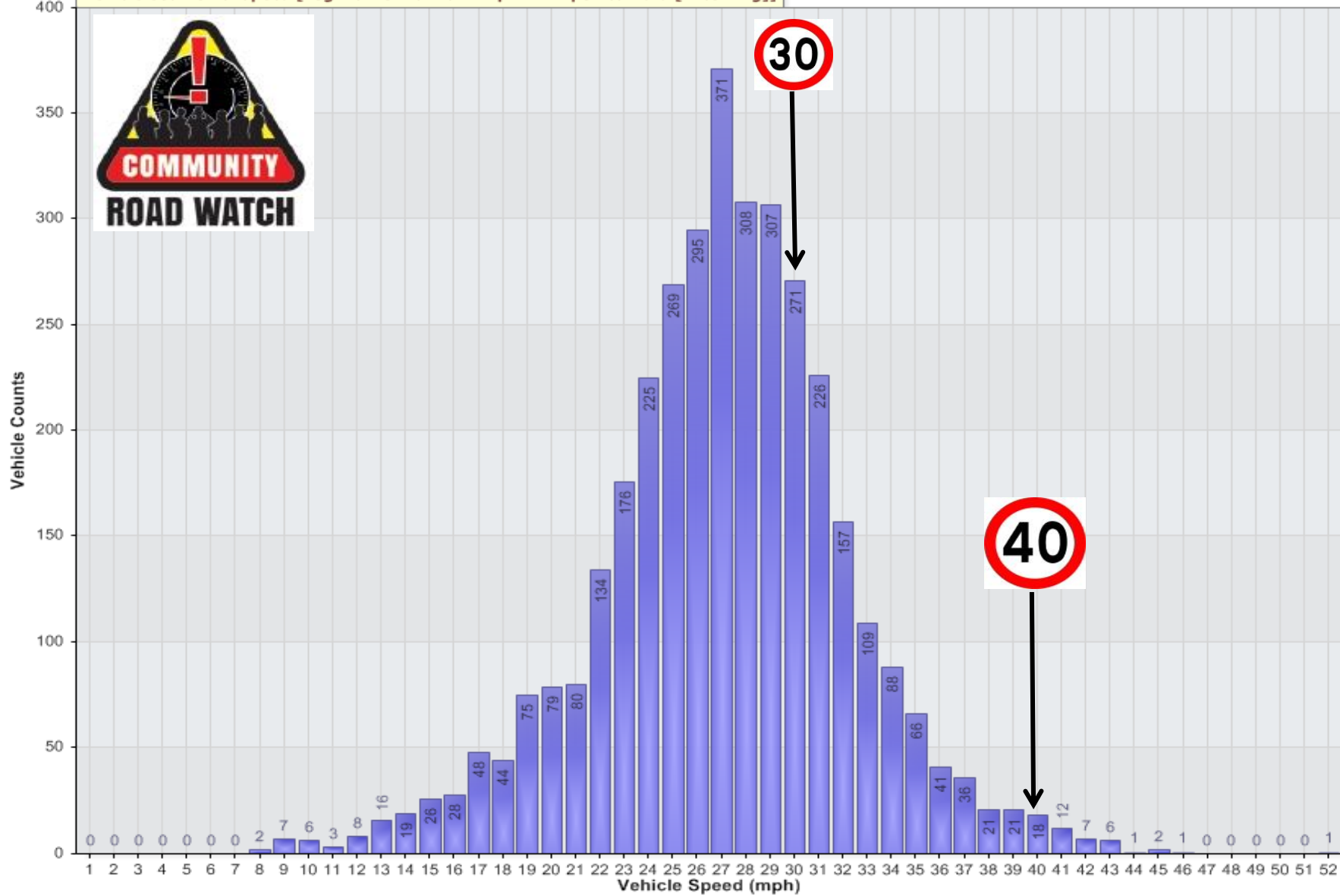
Vehicle Counts Vs. Speed [LogELS-BoxRdAtGnD-Apr22: Imported Data [Incoming]]
