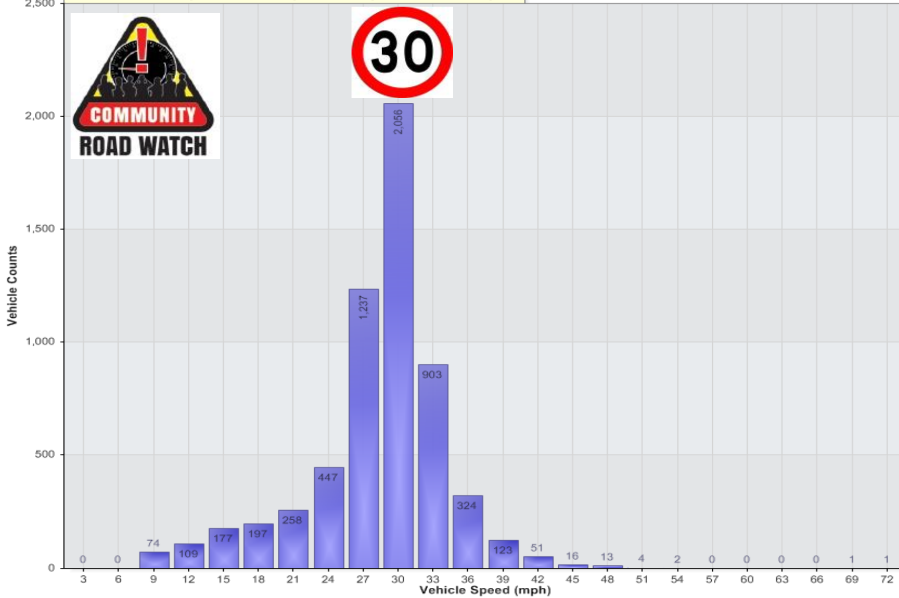
Vehicle Counts Vs. Speed [DES-SID-UphillOct20: Uphill towards Veasey Rd]
