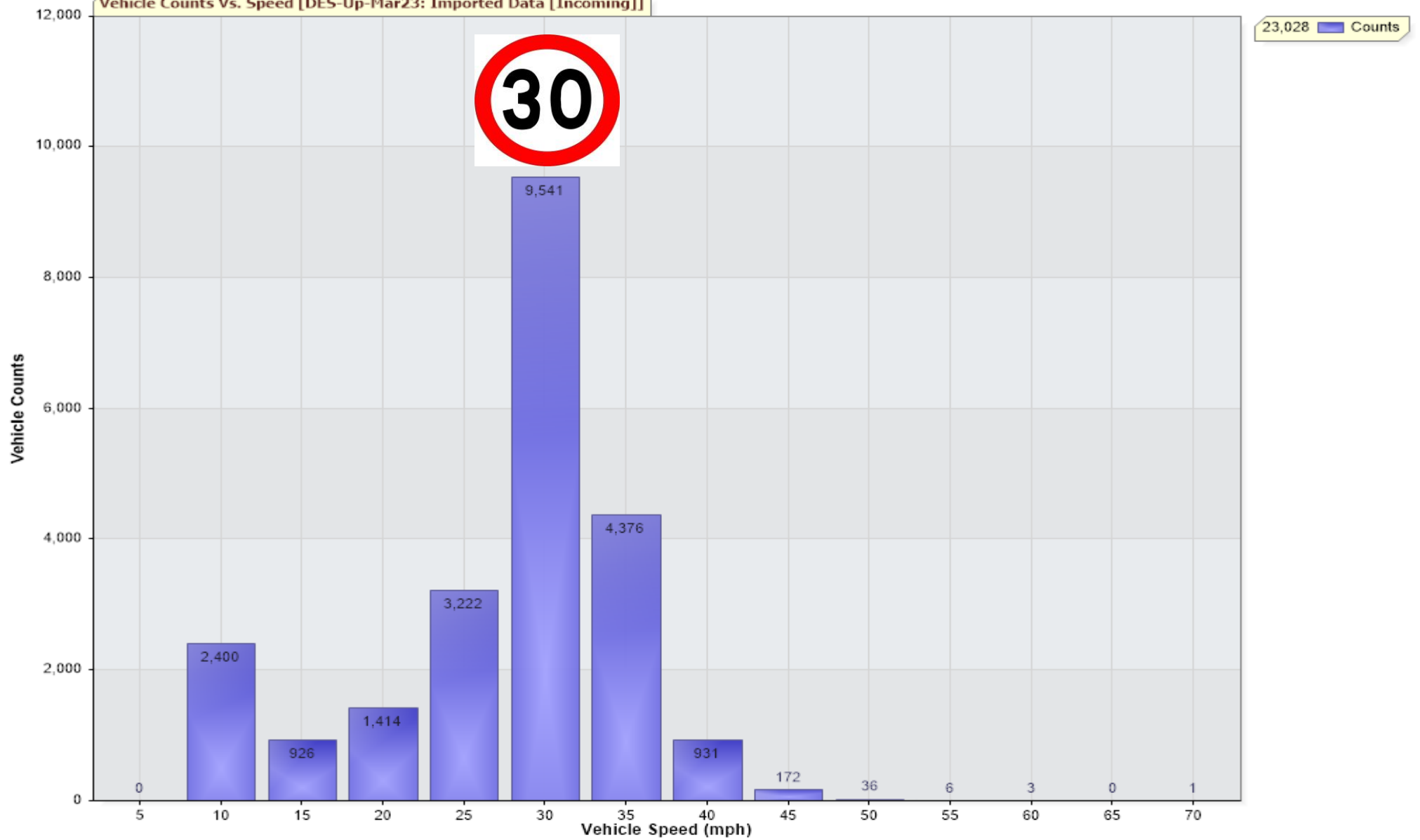
Vehicle Counts Vs. Speed [DES-Up-Mar23: Imported Data [Incoming]]
