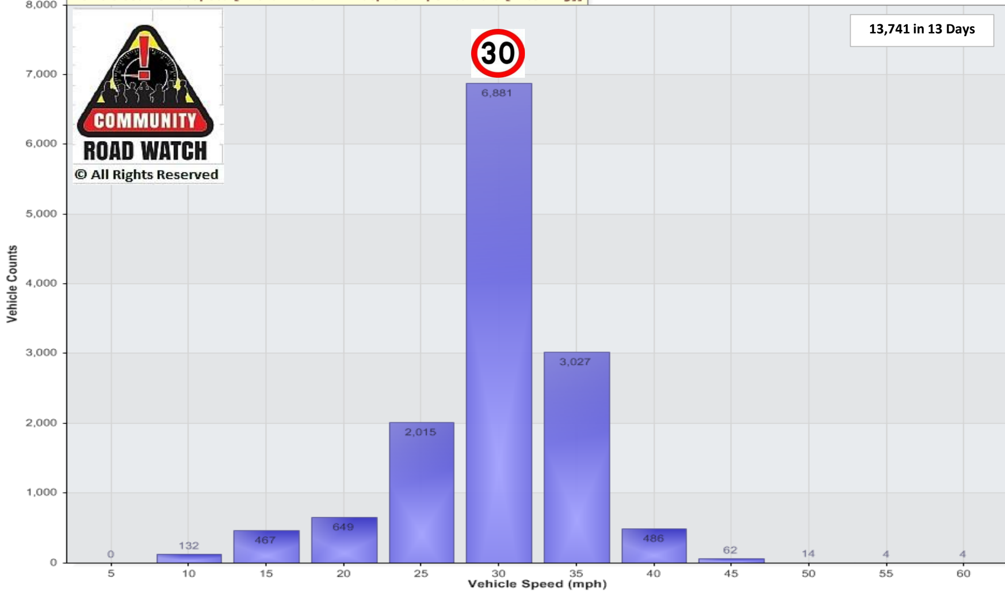
Vehicle Counts Vs. Speed [DES-SID-Downhill-Sep20: Imported Data [Incoming]]
