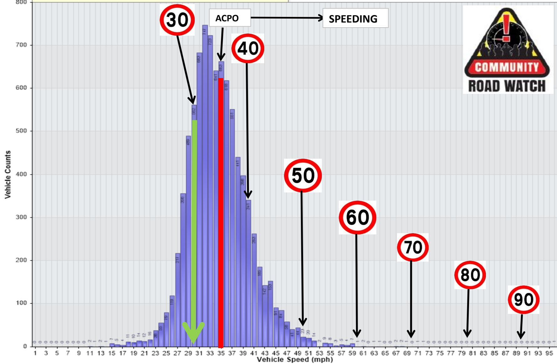
Vehicle Counts Vs. Speed [LogCON-ColneRd-Aug23: Incoming Direction]
