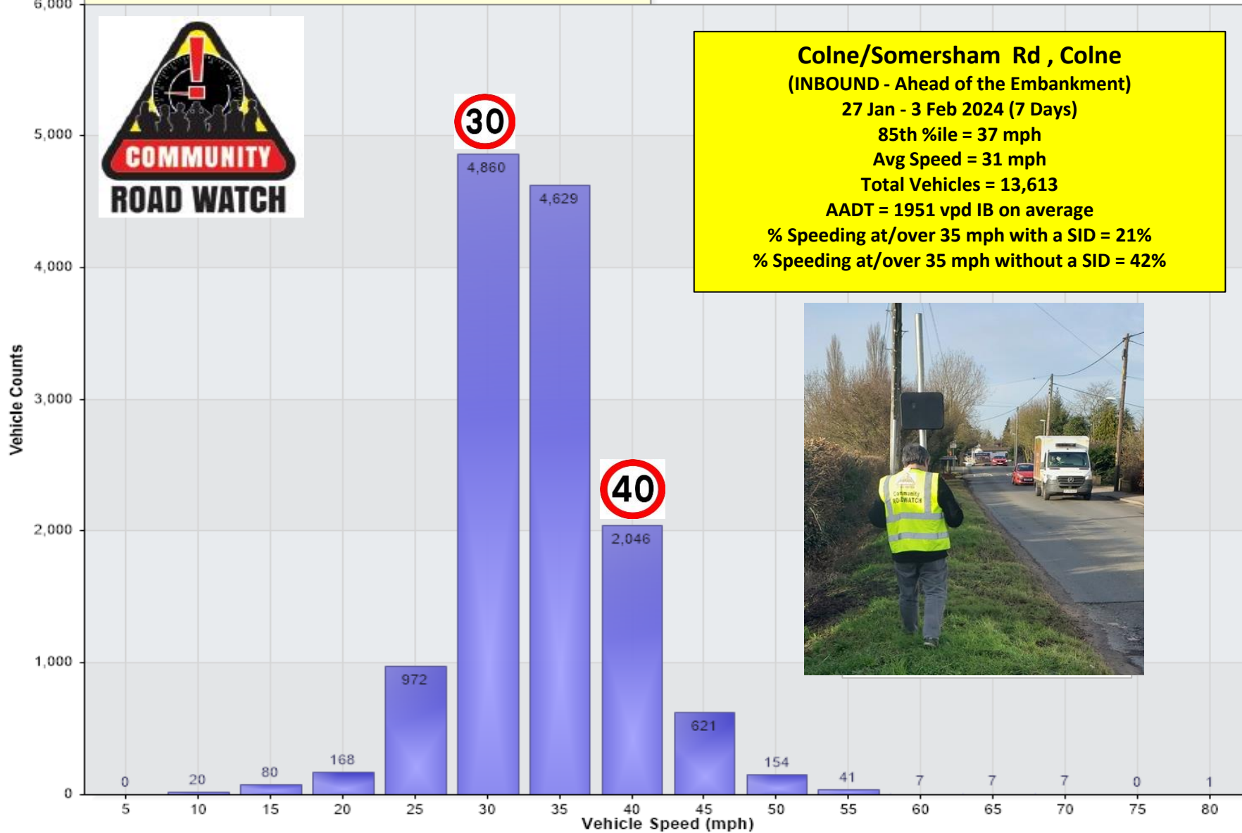
Vehicle Counts Vs. Speed [CON-ColnRd-IB-Feb24: Incoming Direction]
