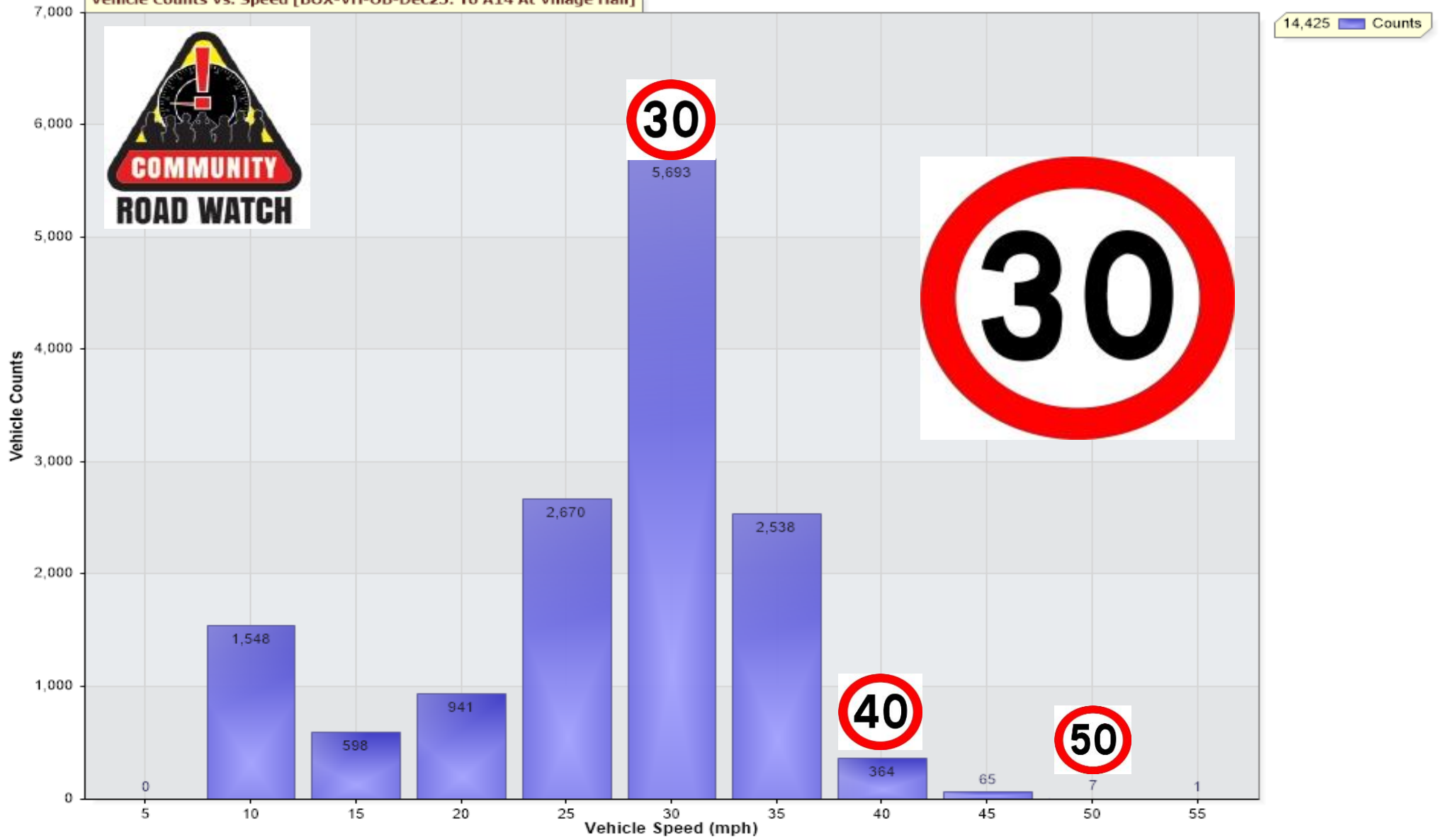
Vehicle Counts Vs. Speed [BOX-VH-OB-Dec23: To A14 At Village Hall]
