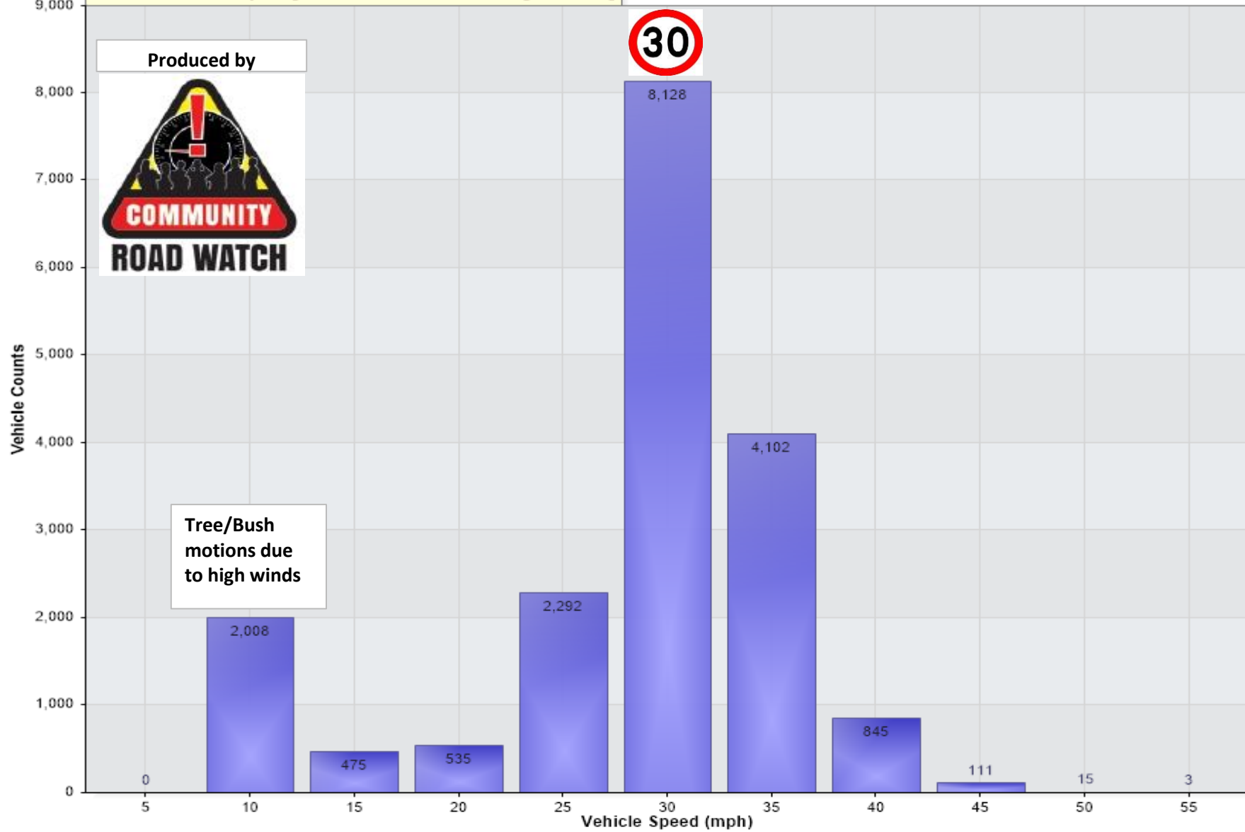
Vehicle Counts Vs. Speed [BOX-SEA-IB-Jan24: Incoming Direction]
