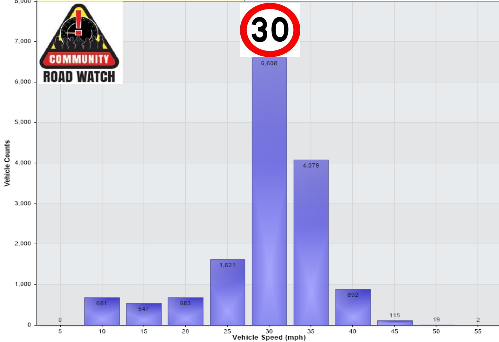
Vehicle Counts Vs. Speed [BOX-SEA-IB-Sep22: In from A14 ]
