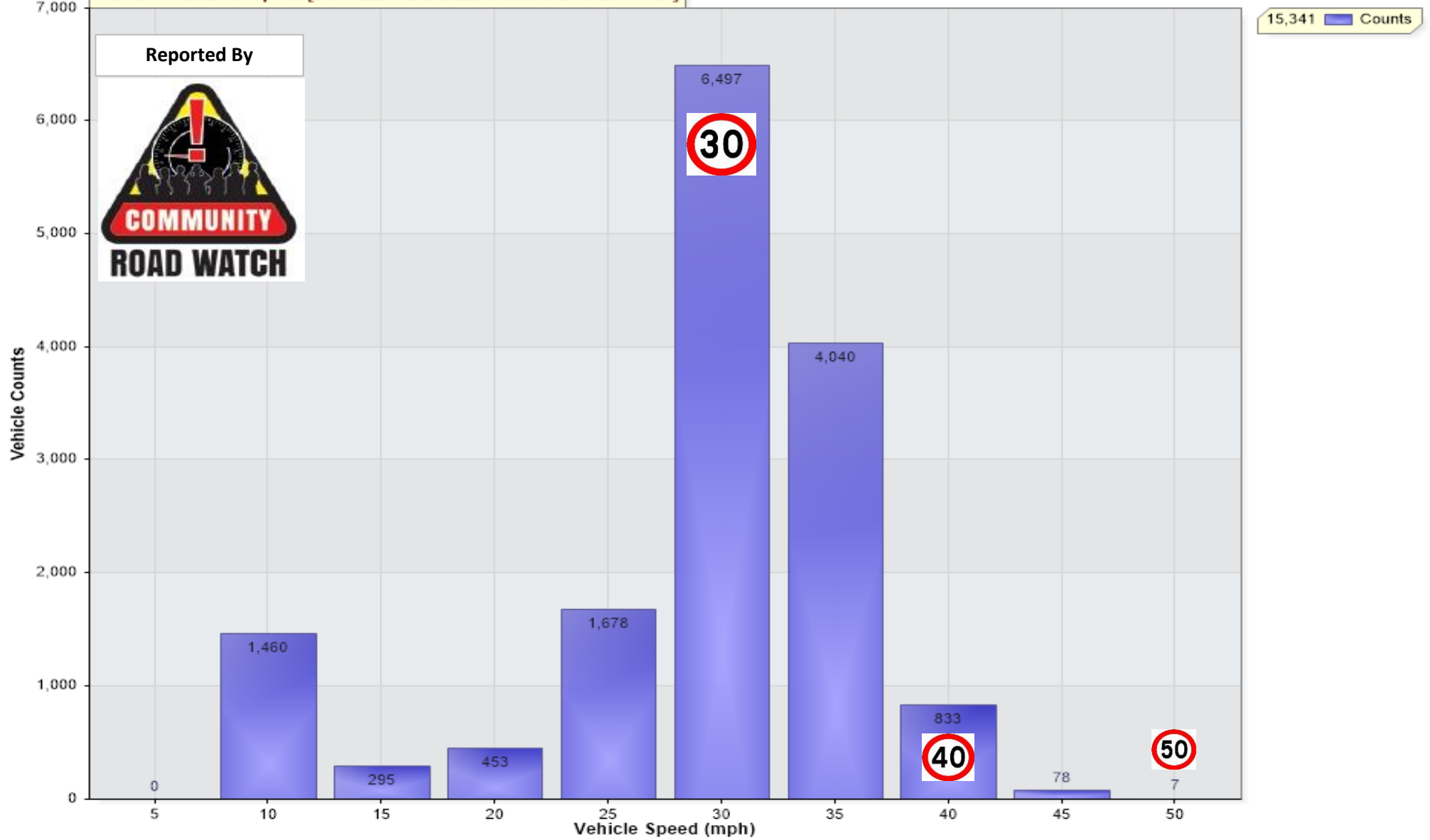
Vehicle Counts Vs. Speed [BOX-ELS-OB-Dec22: Outbound To Elsworth]
