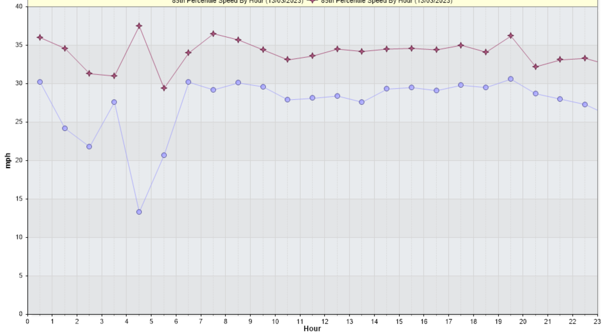
To Elsworth: Average Hourly WEEKDAY Speeds for Week of 13/03/2023 Average Hourly WEEKDAY Speeds By Hour (13/03/2023) — Average Hourly WEEKDAY Speeds By Hour (13/03/2023) 85th Percentile Speed By Hour (13/03/2023) — 85th Percentile Speed By Hour (13/03/2023)
