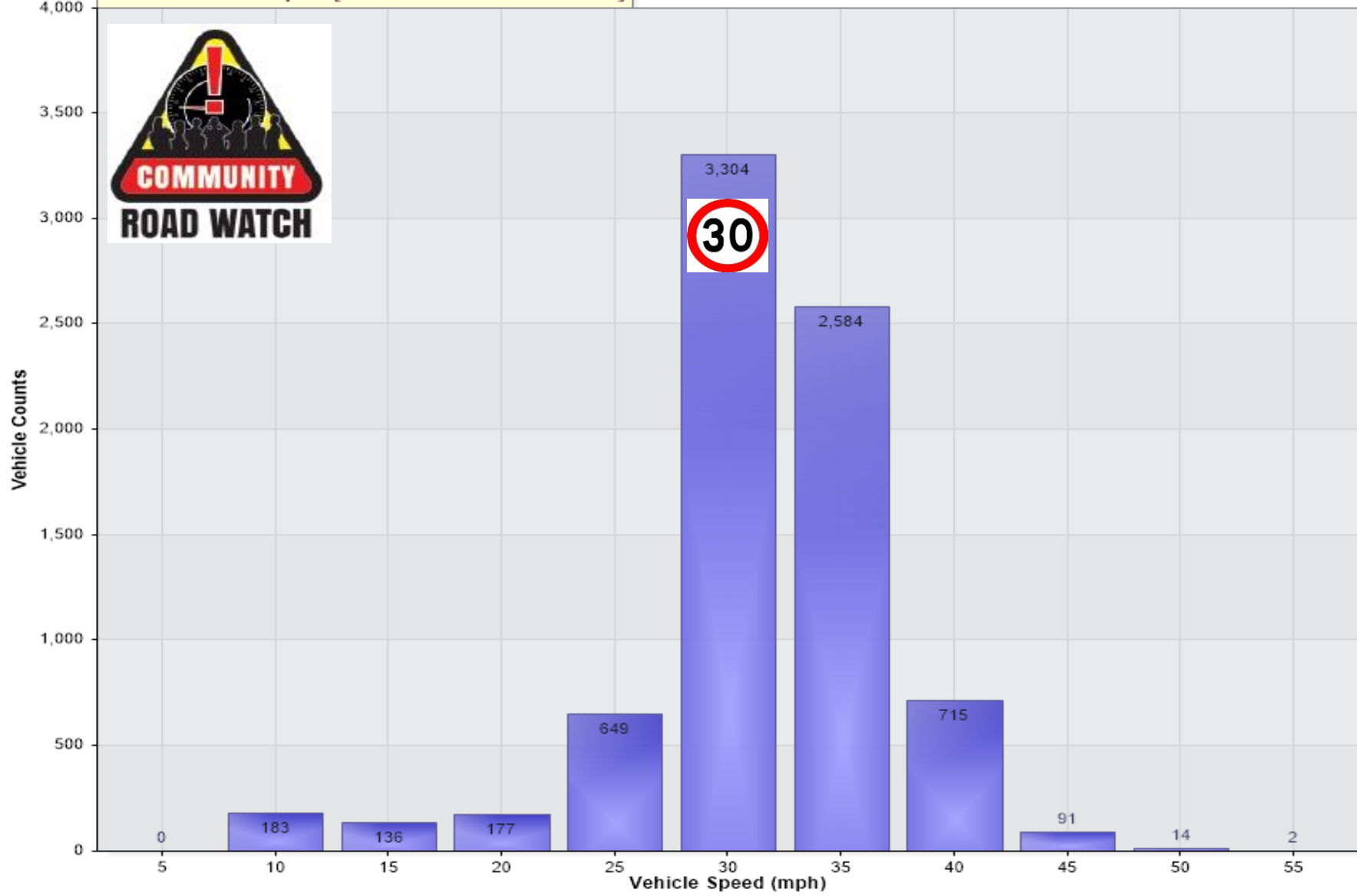
Vehicle Counts Vs. Speed [BOX-ELS-OB-Feb24: Outbound]
